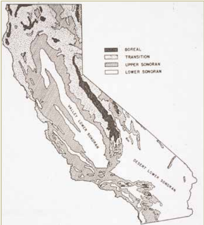
Life zones of California
